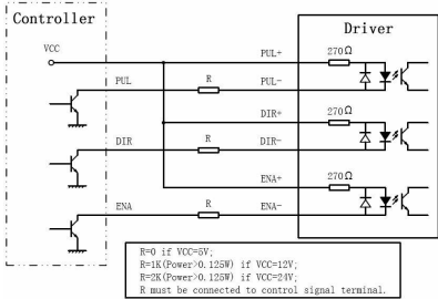
Figure 2: Connections to open-collector signal (common-anode)
