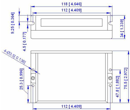
Figure 1: Mechanical specifications
