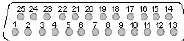
Figure 4 DB25 connector pin assignments
