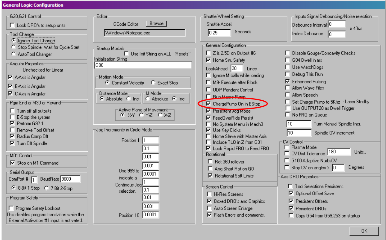
Figure 2: Mach3 general settings dialog. Correct chargepump setting circled.
