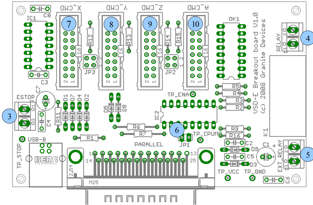
Figure 1: VSDEPI physical overview
