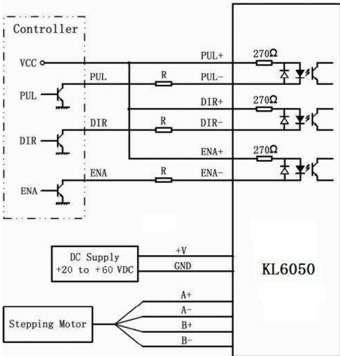
Figure 2: Typical Connections
