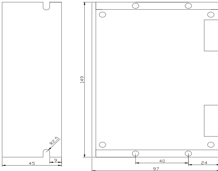
Figure 1: Mechanical Specifications
