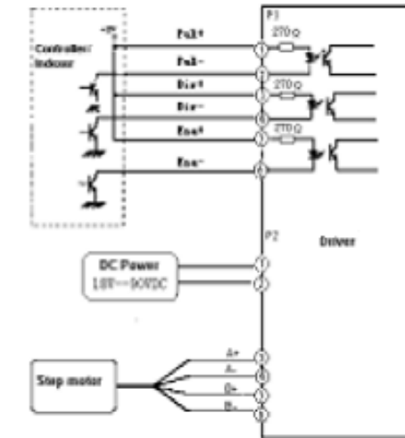
Figure 9: Driver connection in a stepping system
