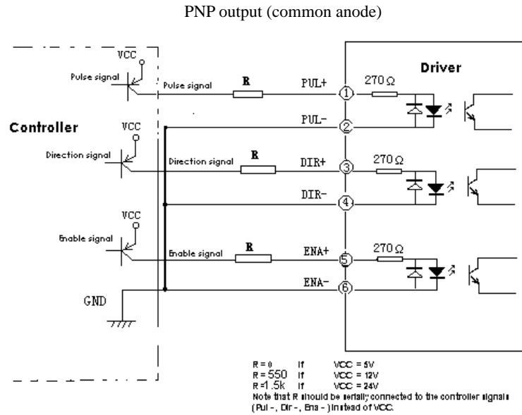
Figure 2: Signal Interface
