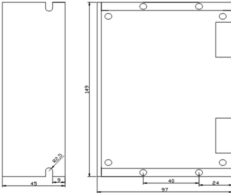
Figure 1: Mechanical Specifications
