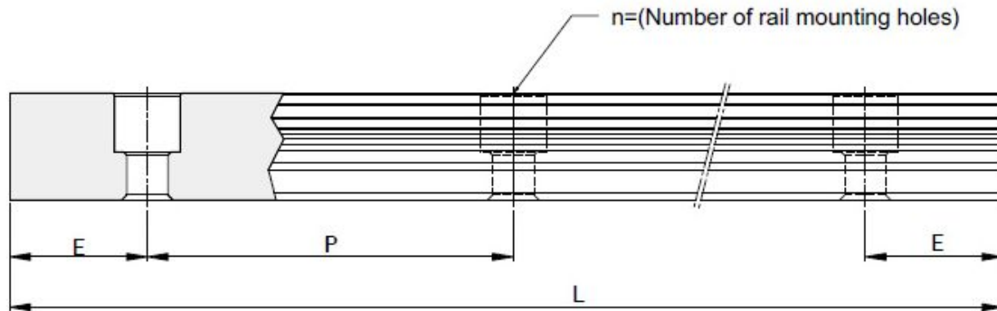
Rail Standard Length and Max. Length
