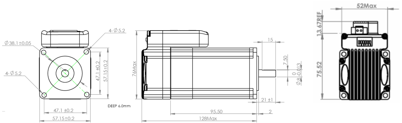
Mechanical Specification of iSV-B23130T-D4
