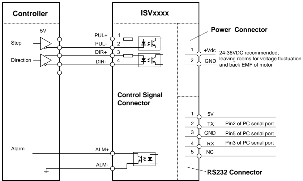
Connect iSV-Bxxx to controller of differential output
