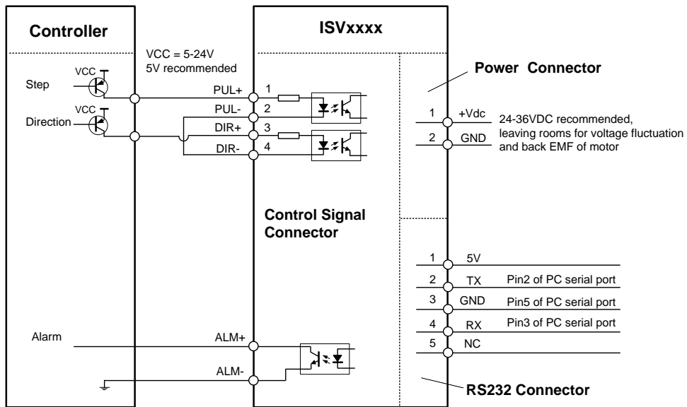
Connect iSV-Bxxx to controller of sourcing output
