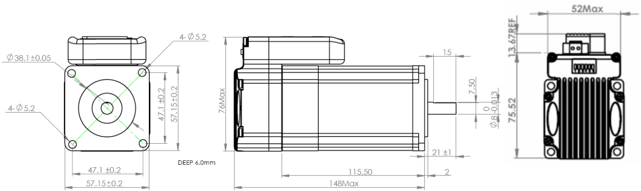
Mechanical Specification of iSV-B23180T-D4
