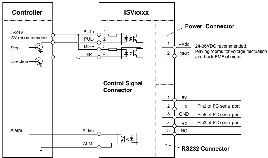
Connect iSV-Bxxx to controller of sinking output
