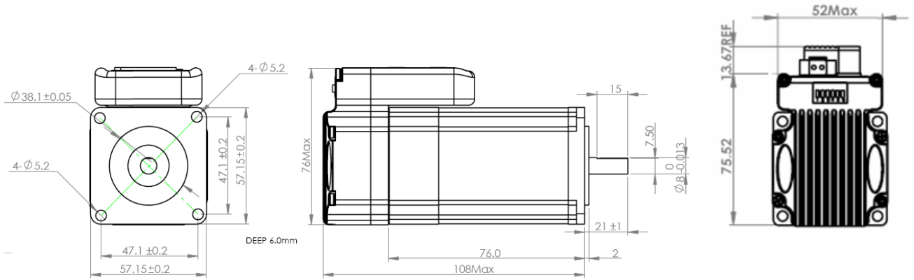
Mechanical Specification of iSV-B23090T-D4
